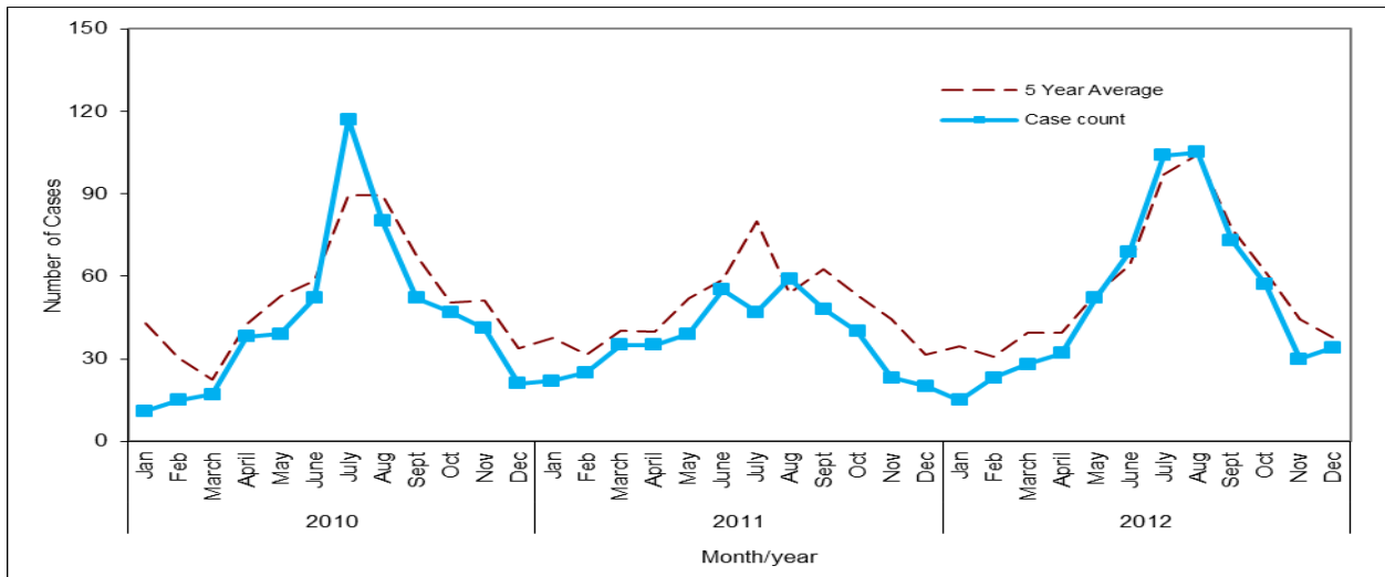
Figure 22. Salmonellosis cases versus 5 year average baseline by month and year, 2010-2012
