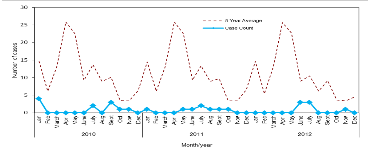
Figure 21. Hepatitis A cases versus 5 year average baseline by month and year, 2010-2012
